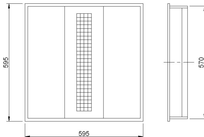
NOMINAL DIMENSIONS IN mm Tolerance +/-5
