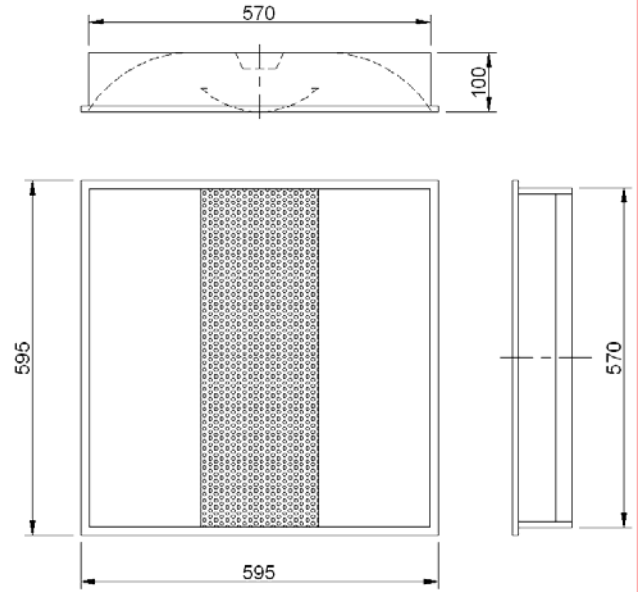
NOMINAL DIMENSIONS IN mm Tolerance +/-5
