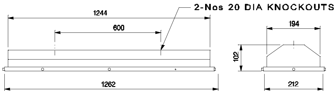
NOMINAL DIMENSIONS IN mm Tolerance +/-5
