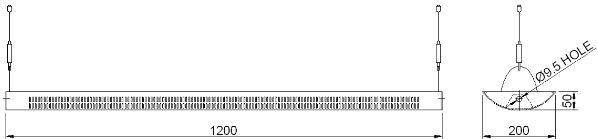
NOMINAL DIMENSIONS IN mm Tolerance +/-5
