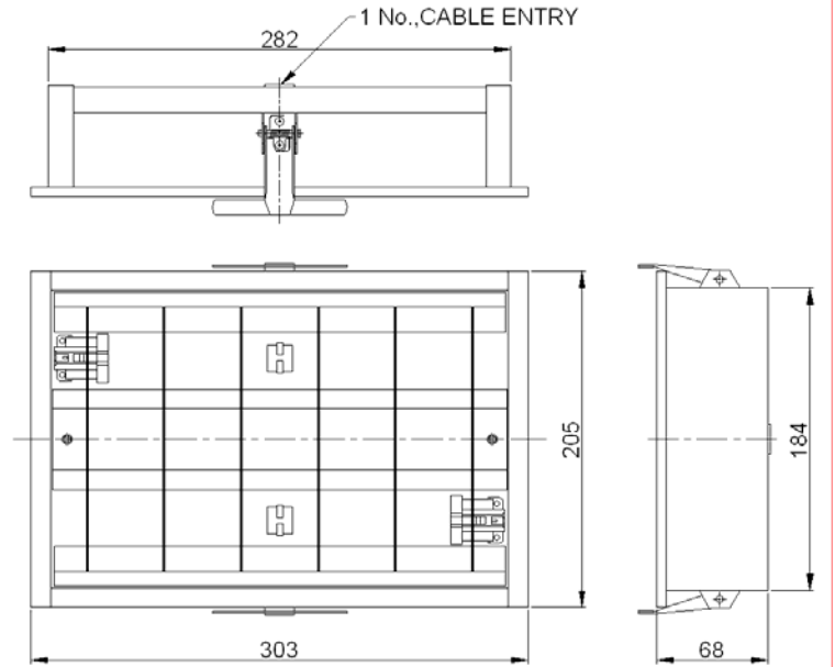
NOMINAL DIMENSIONS IN mm Tolerance +/-5
